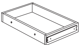
Drawer Box (Assembled) 14" Deep 24", 30" Wide 5", 7 1/2", 10" sizes 19" Deep 24", 30" Wide 7 1/2", 10" sizes Available in white only.
