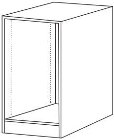
"A" Cabinet 41 1/8" H x 25 1/2" W x 31 3/4" D. *Colors available.
